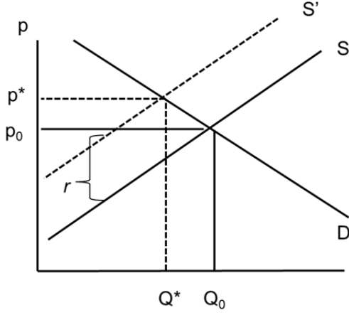
(a) Federal coal only, no emissions regulation
